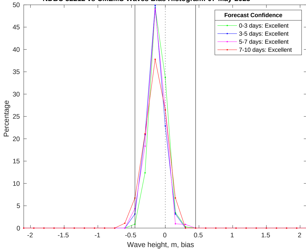
NDBC 52212 vs CMEMS Waves Bias Histogram: 07-May-2025
