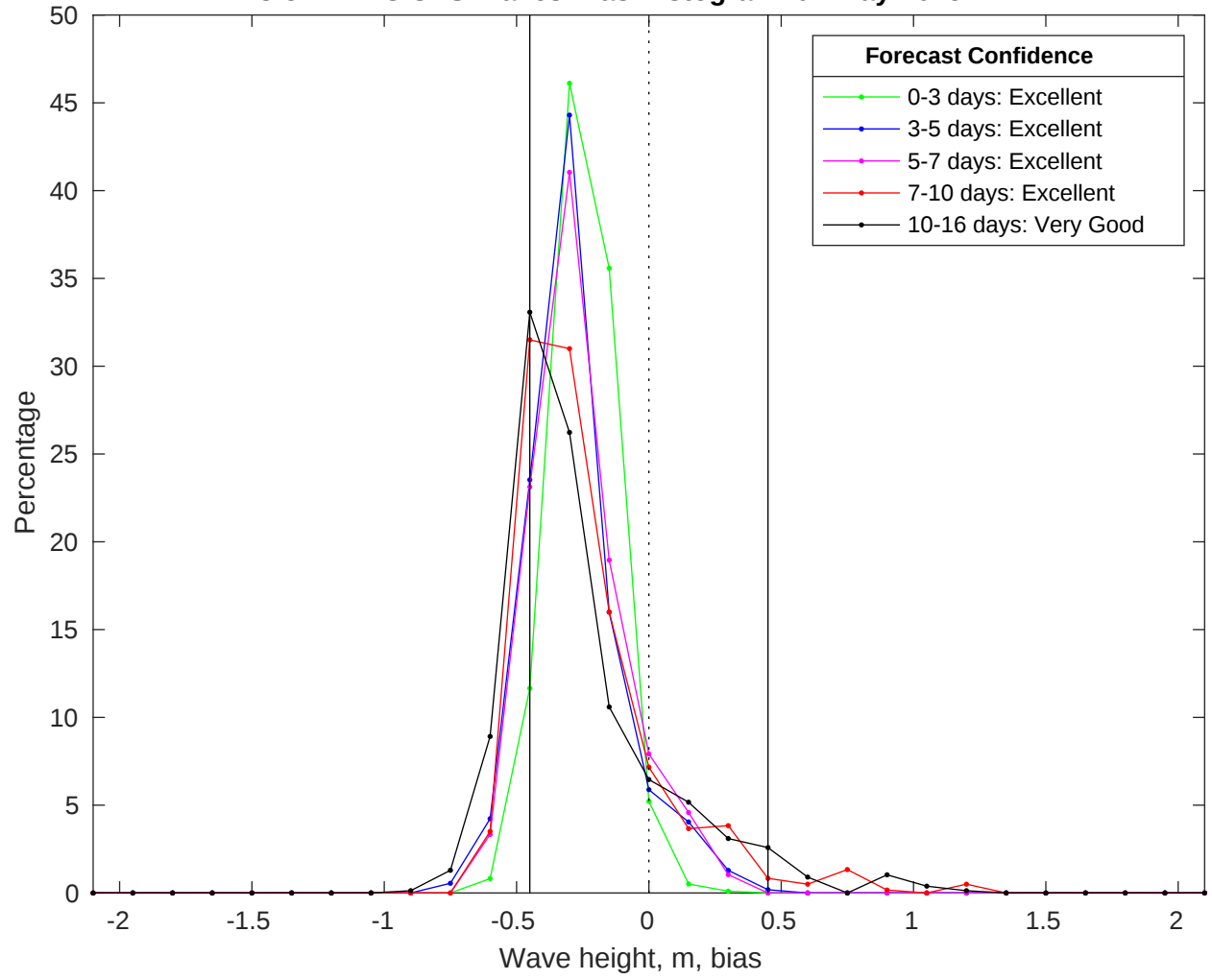
NDBC 52212 vs GFS Waves Bias Histogram: 07-May-2025
