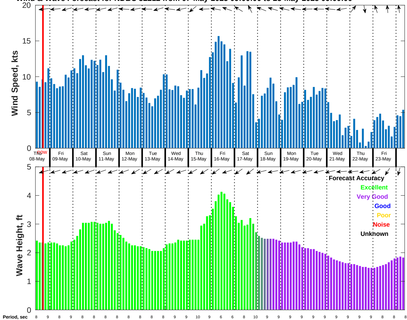
Wind & Wave Forecast for NDBC 52212 from 07-May-2025 09:00:00 to 23-May-2025 09:00:00
