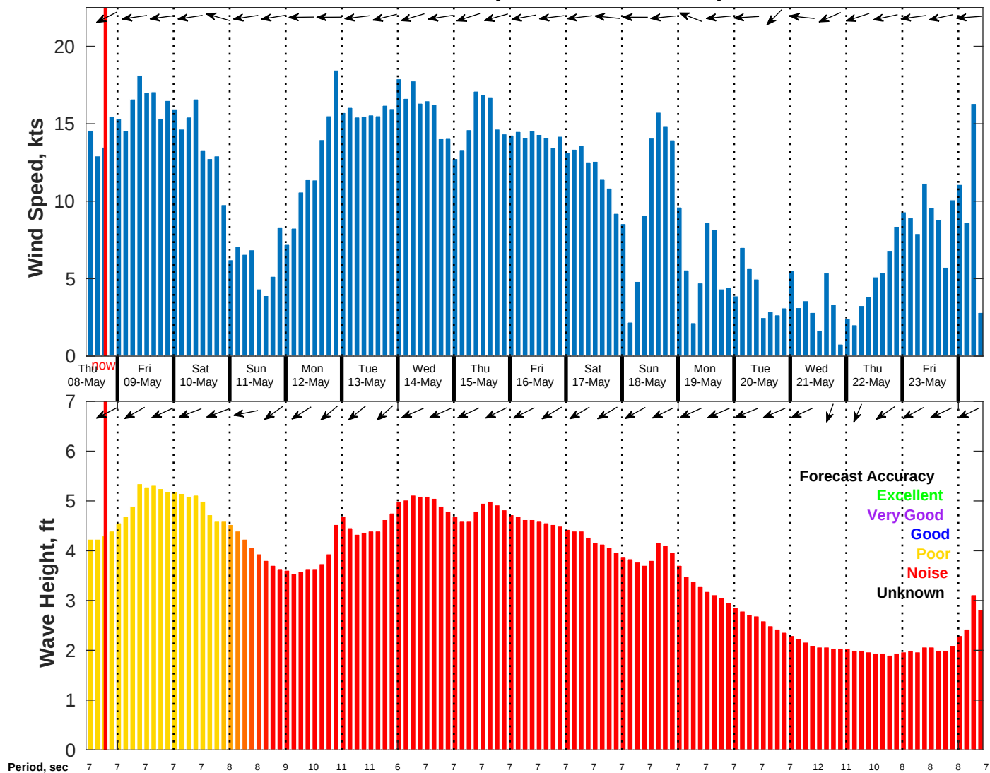
Wind & Wave Forecast for NDBC 52213 from 07-May-2025 11:00:00 to 23-May-2025 11:00:00
