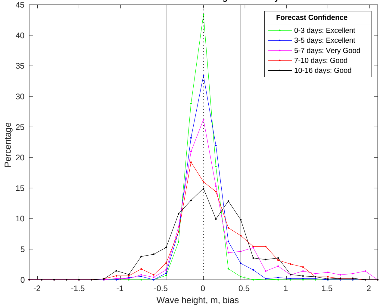
NDBC 41004 vs GFS Waves Bias Histogram: 08-May-2025
