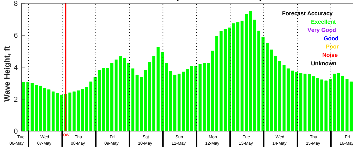
CMEMS Wave Forecast for NDBC 41004 from 06-May-2025 19:00:00 to 16-May-2025 19:00:00
