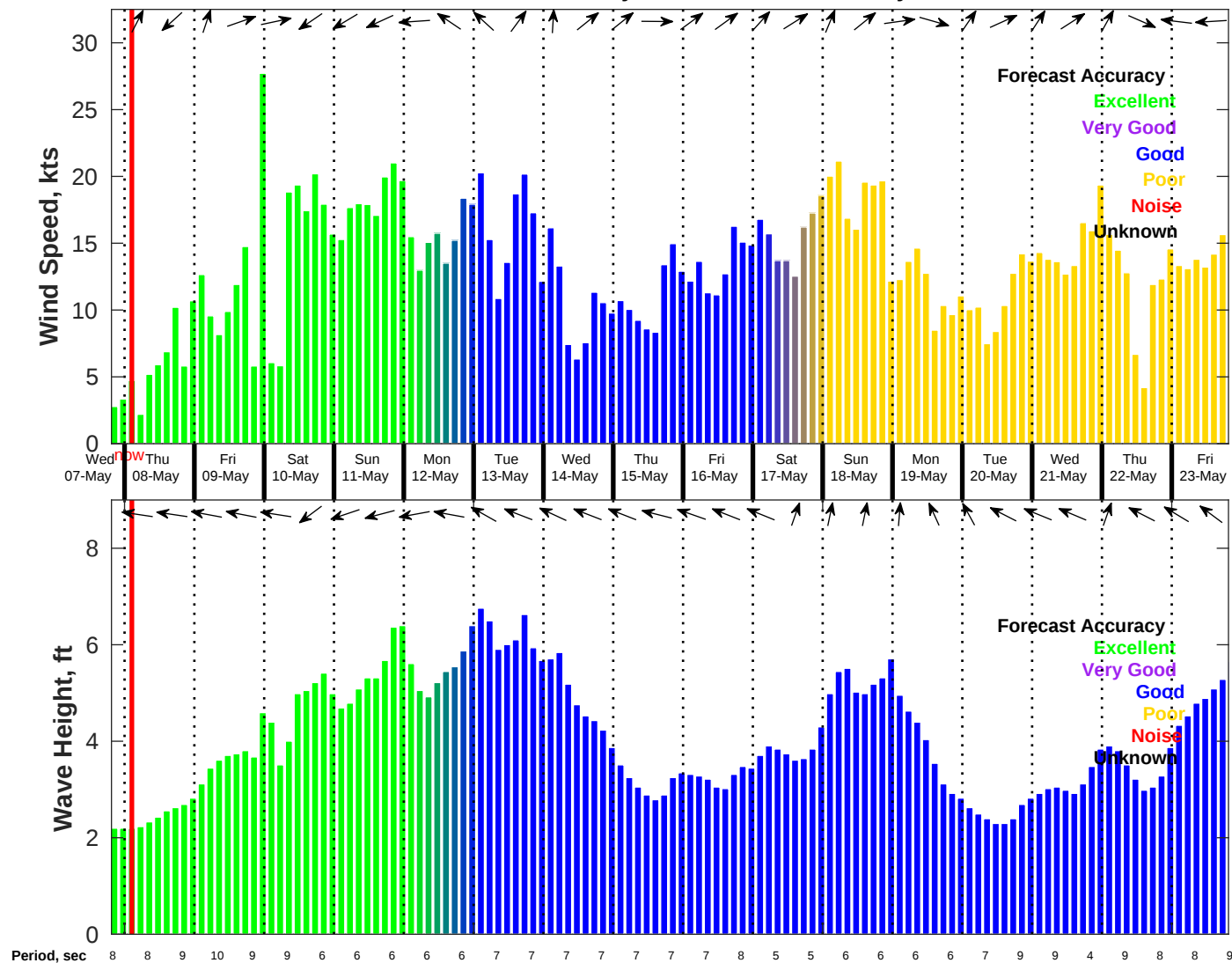
Wind & Wave Forecast for NDBC 41004 from 07-May-2025 19:00:00 to 23-May-2025 19:00:00
