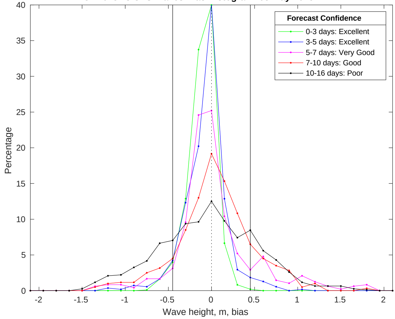
NDBC 41013 vs GFS Waves Bias Histogram: 08-May-2025
