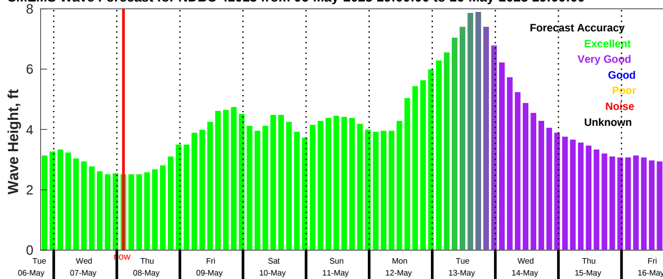
CMEMS Wave Forecast for NDBC 41013 from 06-May-2025 19:00:00 to 16-May-2025 19:00:00
