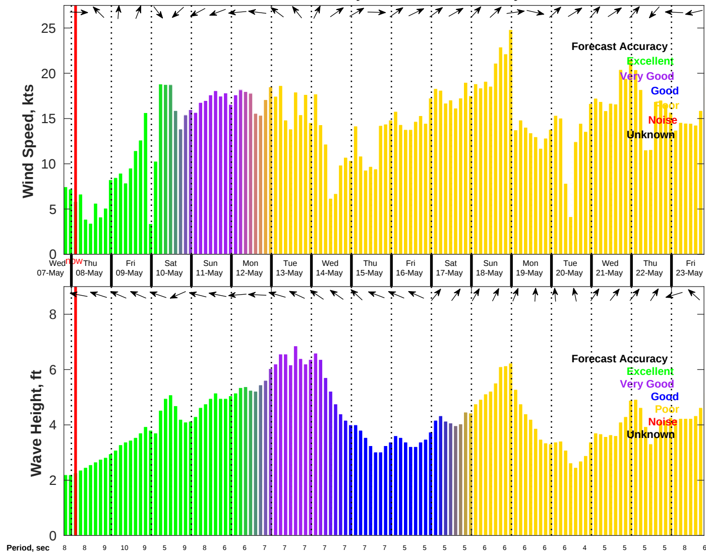
Wind & Wave Forecast for NDBC 41013 from 07-May-2025 19:00:00 to 23-May-2025 19:00:00
