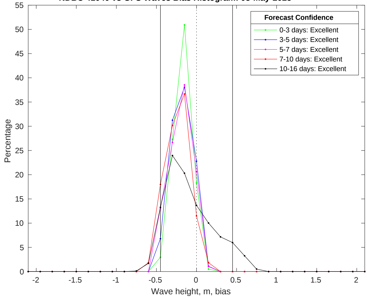
NDBC 41040 vs GFS Waves Bias Histogram: 08-May-2025
