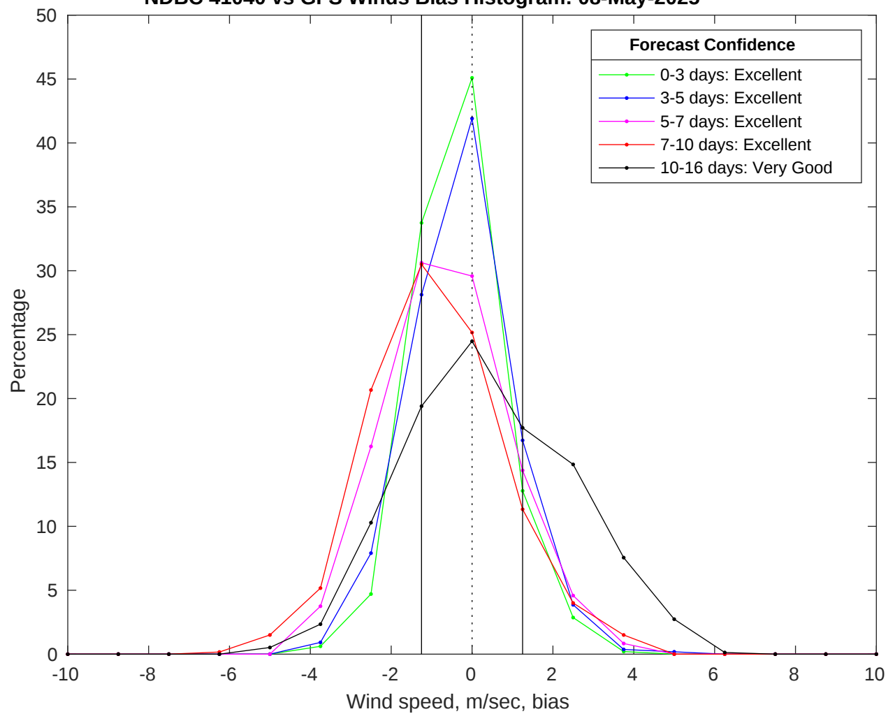
NDBC 41040 vs GFS Winds Bias Histogram: 08-May-2025
