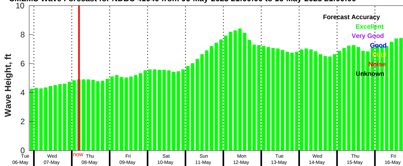
CMEMS Wave Forecast for NDBC 41040 from 06-May-2025 21:00:00 to 16-May-2025 21:00:00
