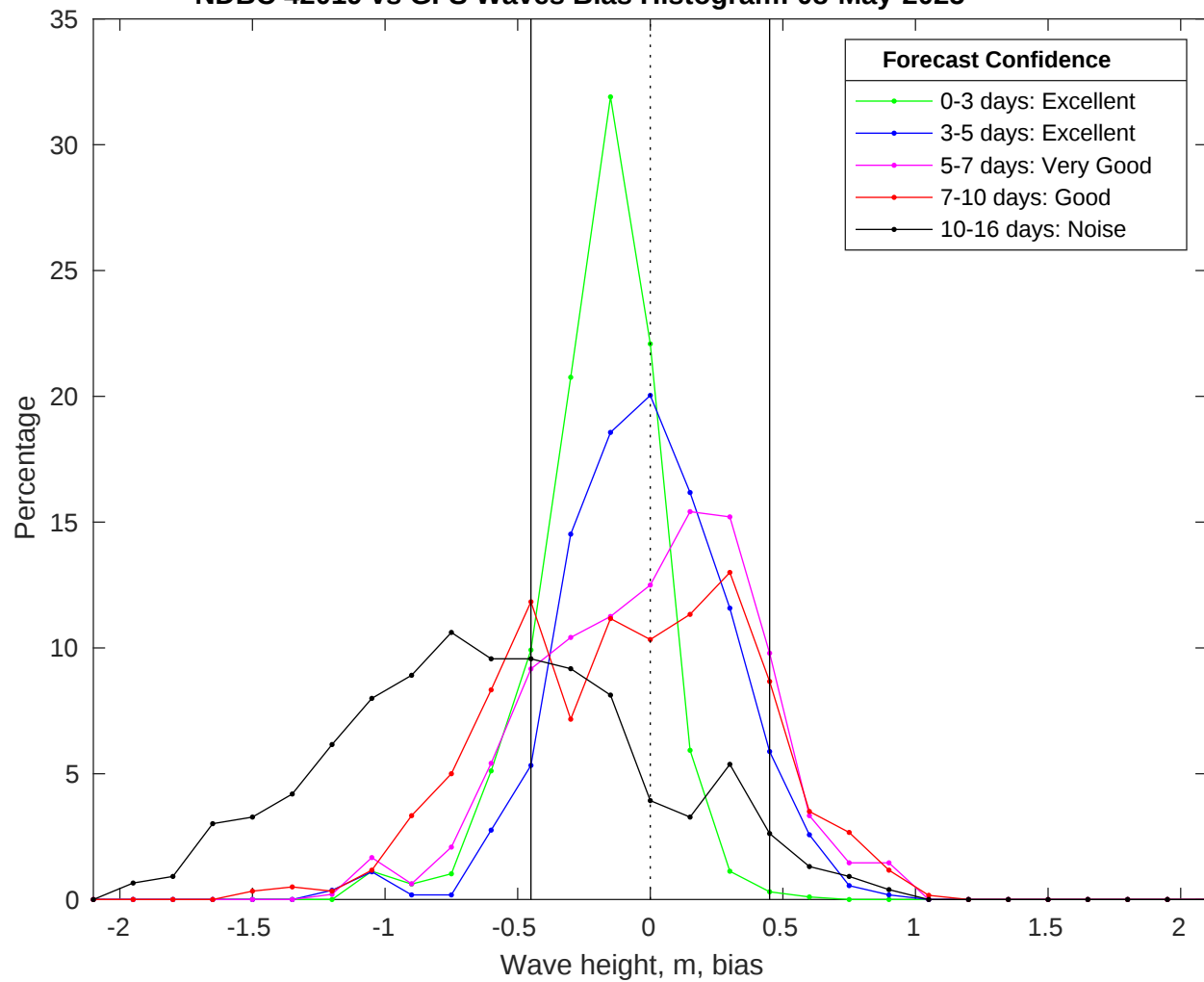
NDBC 42019 vs GFS Waves Bias Histogram: 08-May-2025
