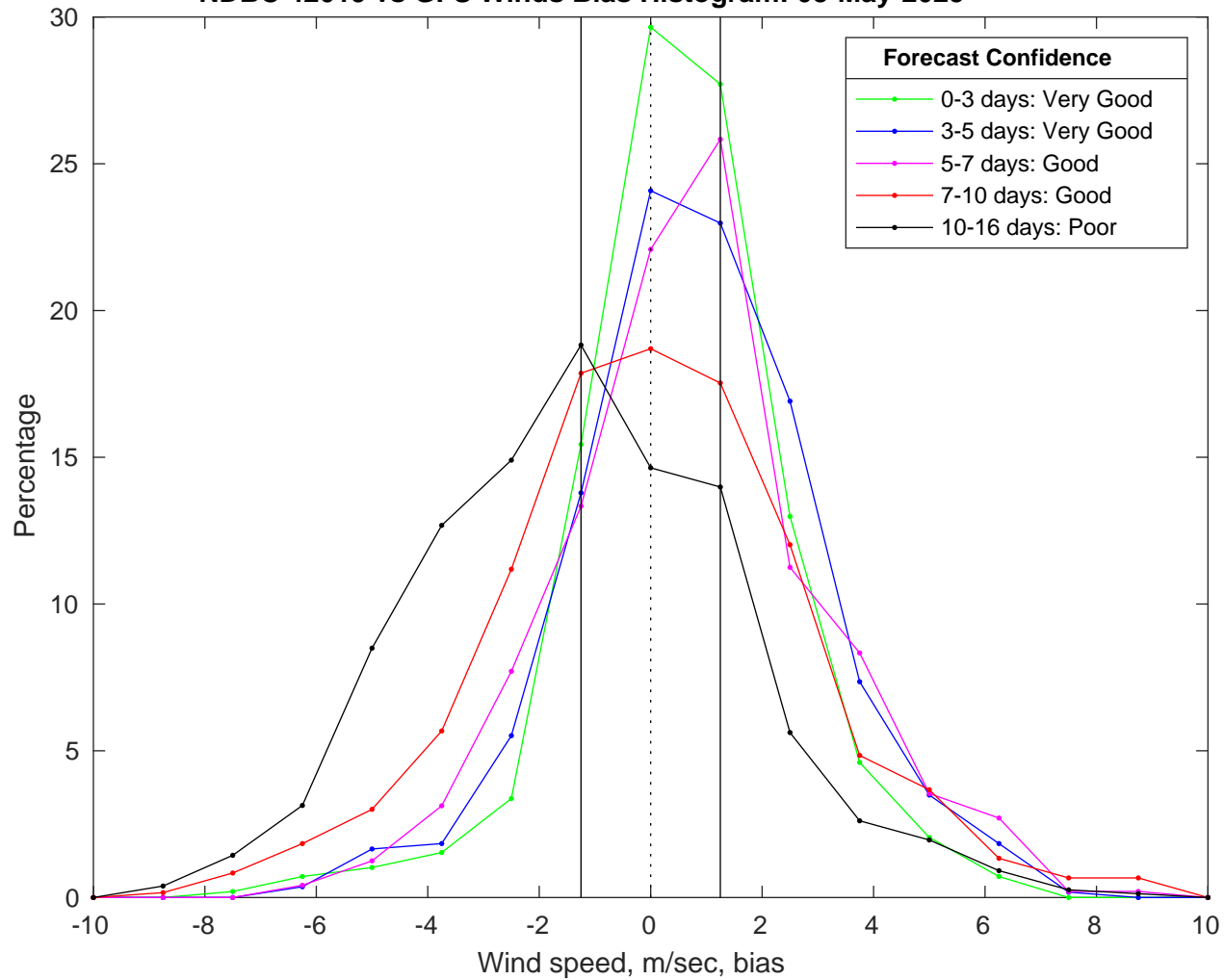
NDBC 42019 vs GFS Winds Bias Histogram: 08-May-2025
