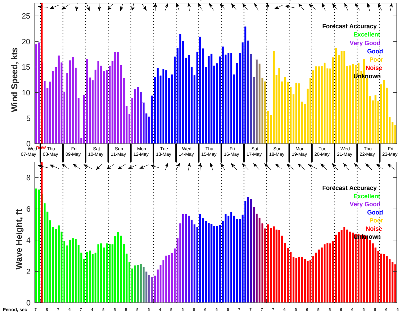
Wind & Wave Forecast for NDBC 42019 from 07-May-2025 18:00:00 to 23-May-2025 18:00:00
