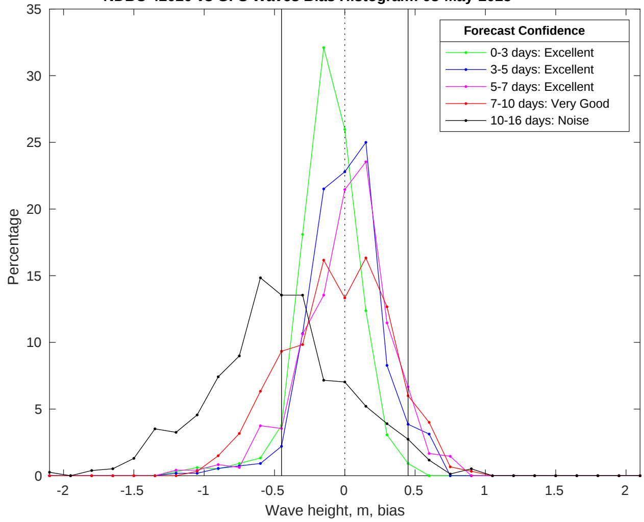
NDBC 42020 vs GFS Waves Bias Histogram: 08-May-2025
