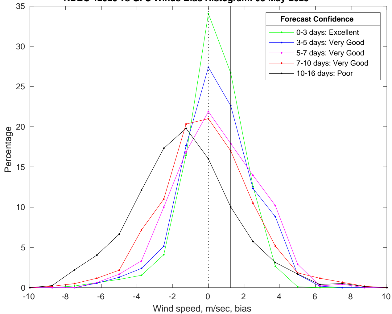
NDBC 42020 vs GFS Winds Bias Histogram: 08-May-2025
