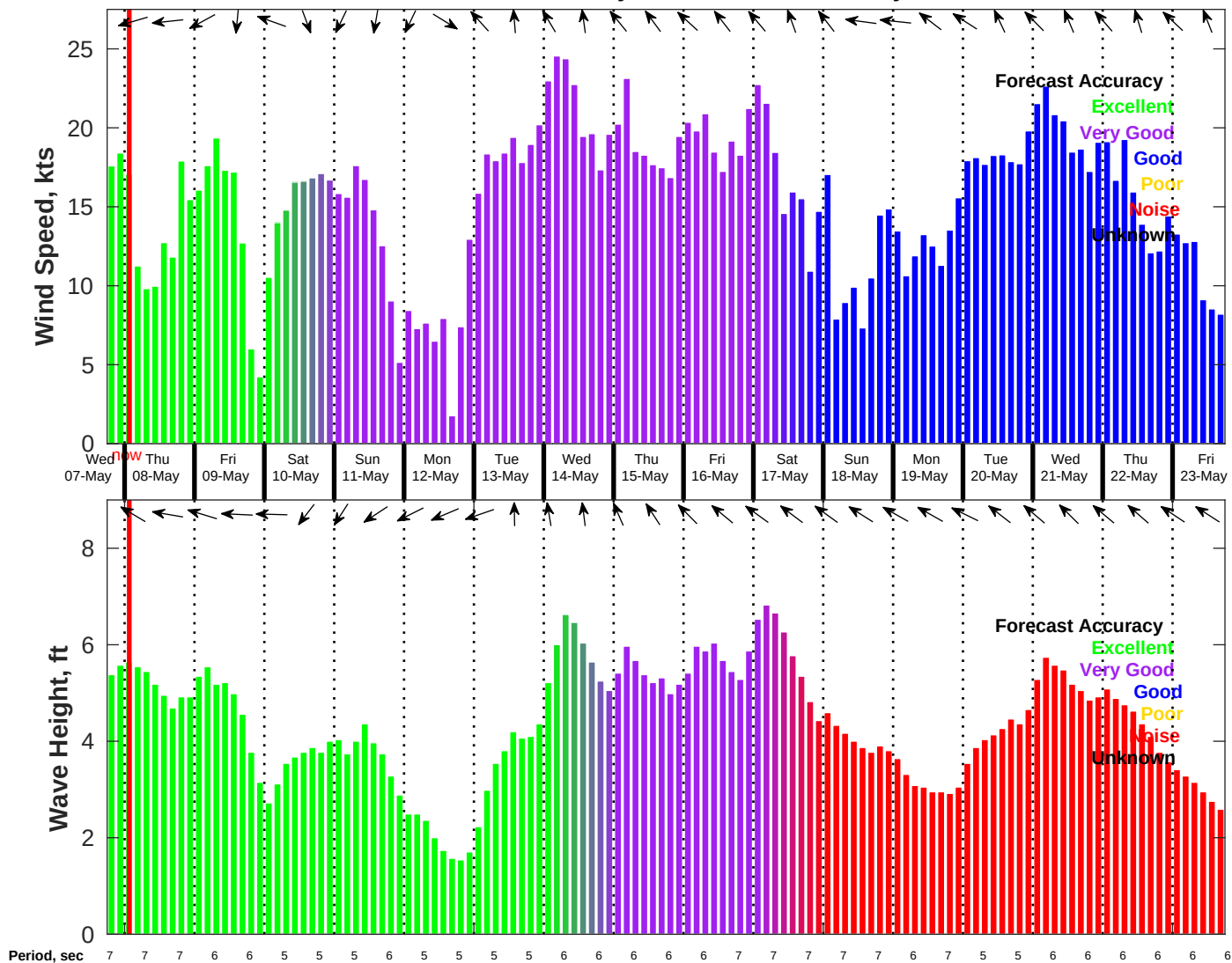
Wind & Wave Forecast for NDBC 42020 from 07-May-2025 18:00:00 to 23-May-2025 18:00:00
