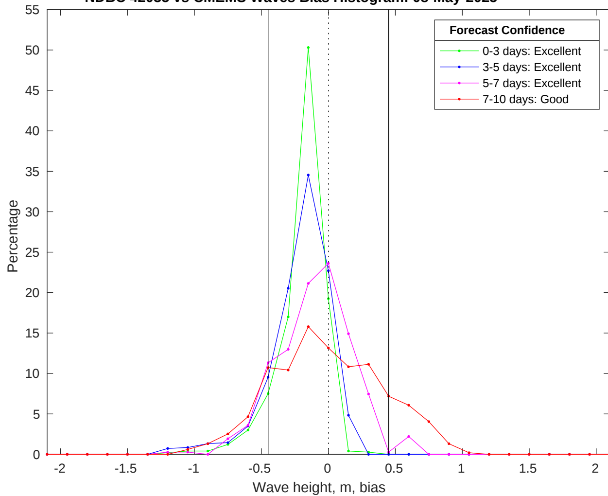
NDBC 42035 vs CMEMS Waves Bias Histogram: 08-May-2025
