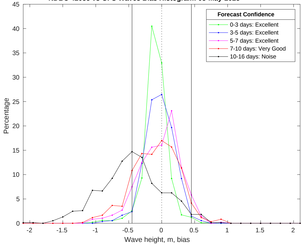
NDBC 42035 vs GFS Waves Bias Histogram: 08-May-2025
