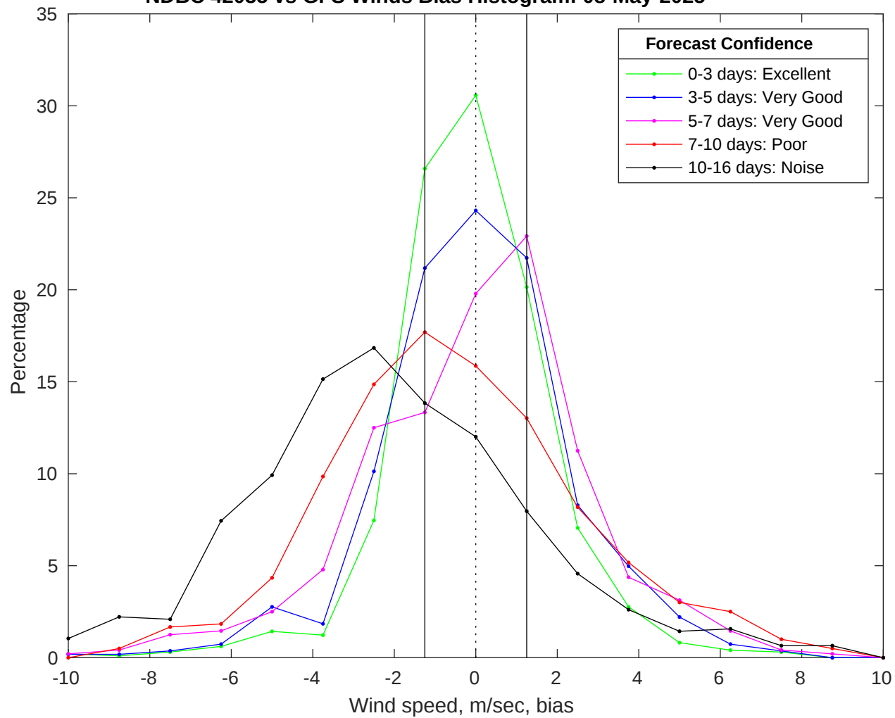
NDBC 42035 vs GFS Winds Bias Histogram: 08-May-2025
