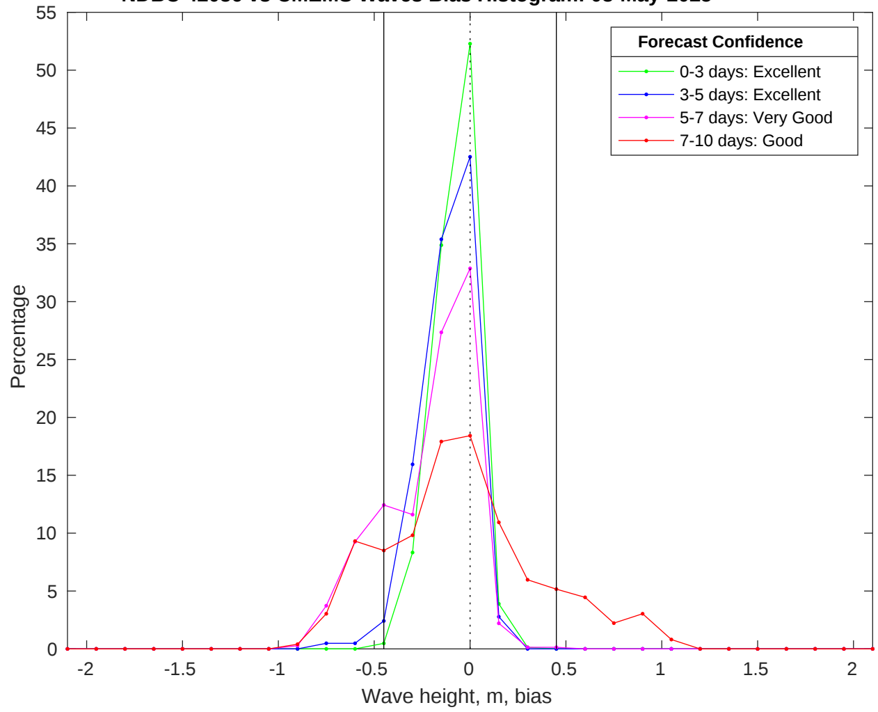
NDBC 42036 vs CMEMS Waves Bias Histogram: 08-May-2025
