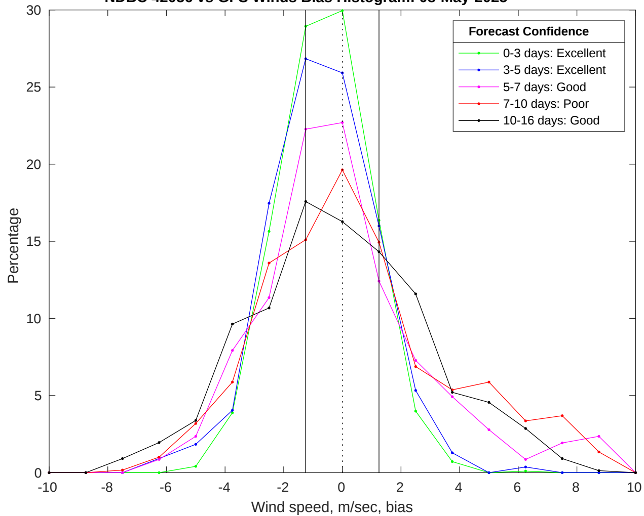
NDBC 42036 vs GFS Winds Bias Histogram: 08-May-2025
