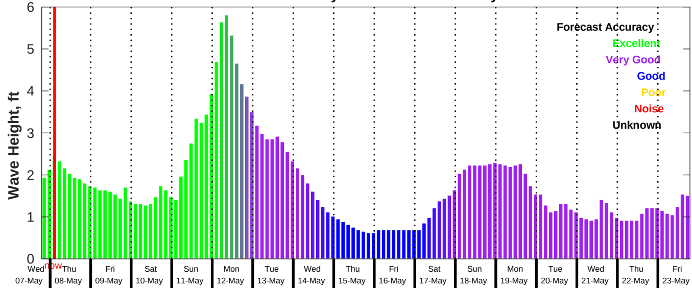
GFS Wave Forecast for NDBC 42036 from 07-May-2025 19:00:00 to 23-May-2025 19:00:00
