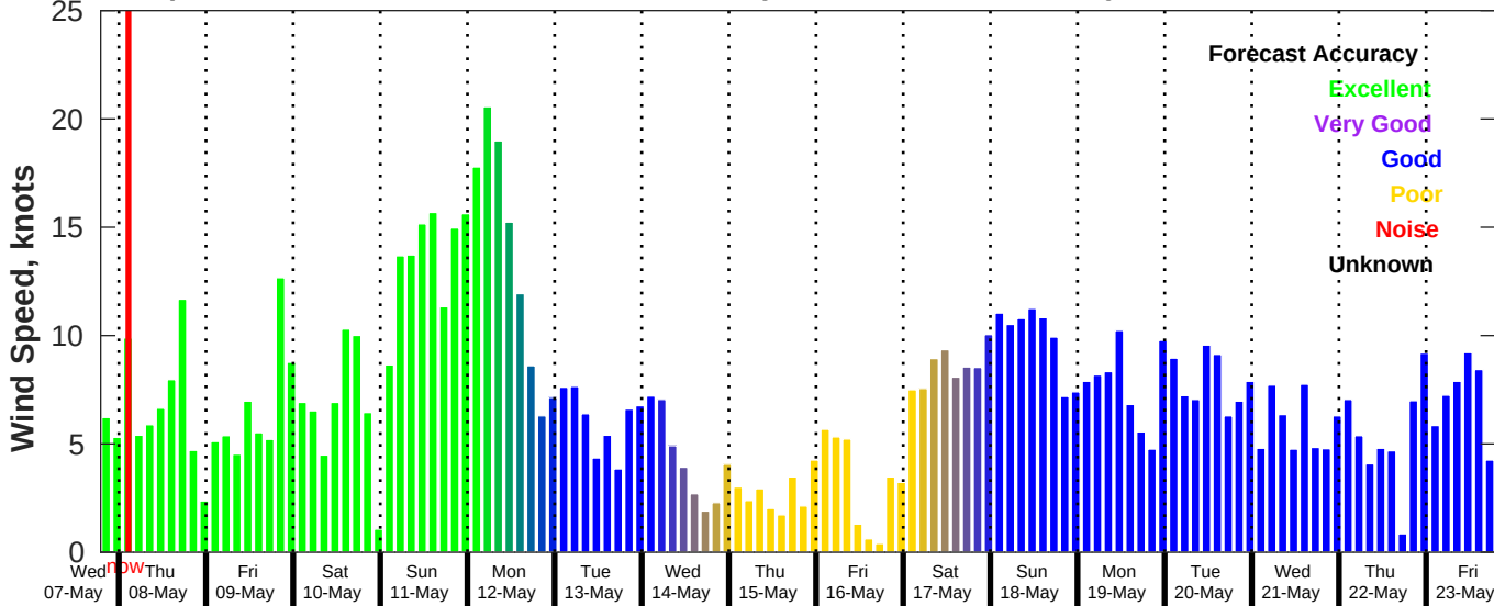
GFS Wind Speed Forecast for NDBC 42036 from 07-May-2025 19:00:00 to 23-May-2025 19:00:00
