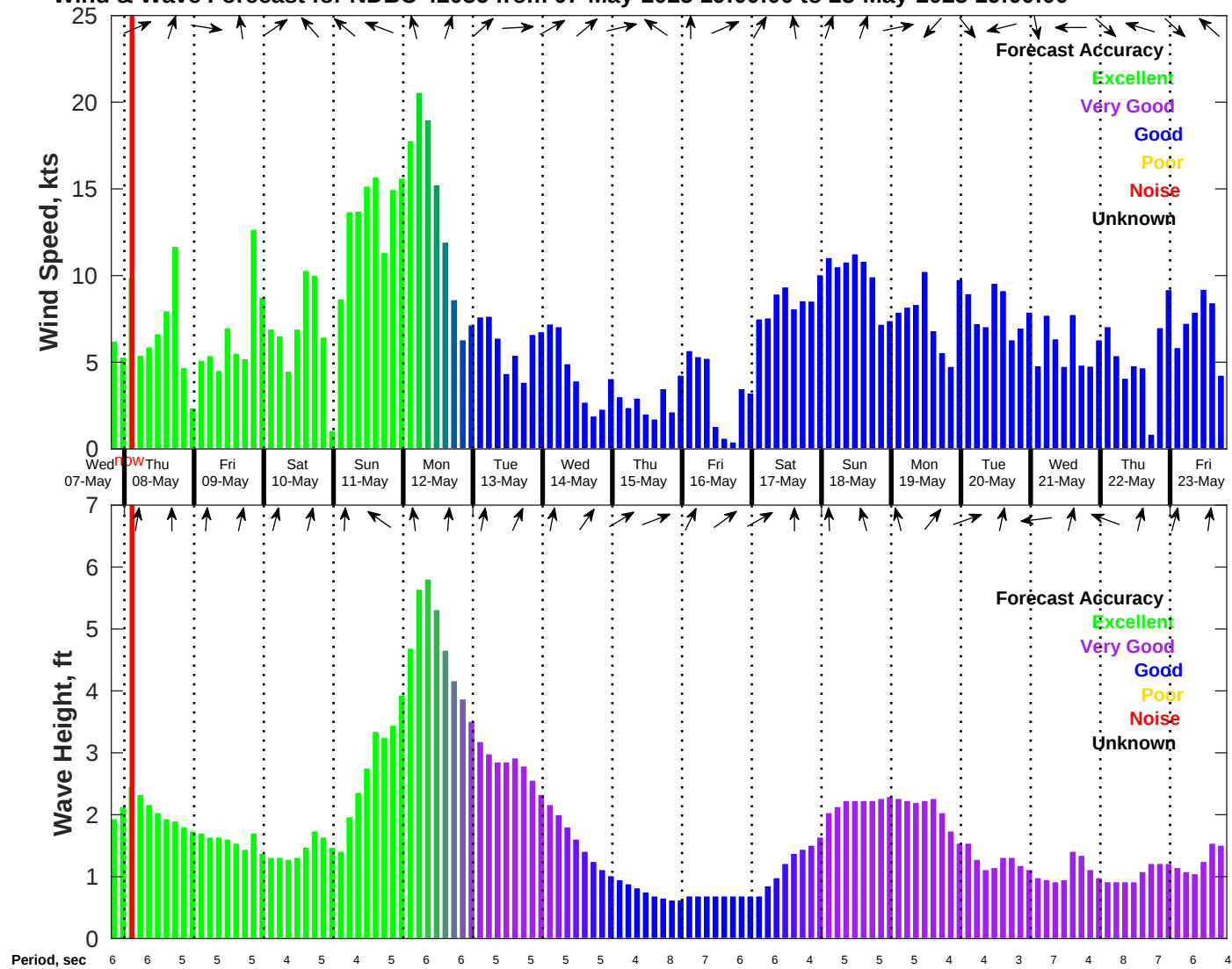
Wind & Wave Forecast for NDBC 42036 from 07-May-2025 19:00:00 to 23-May-2025 19:00:00
