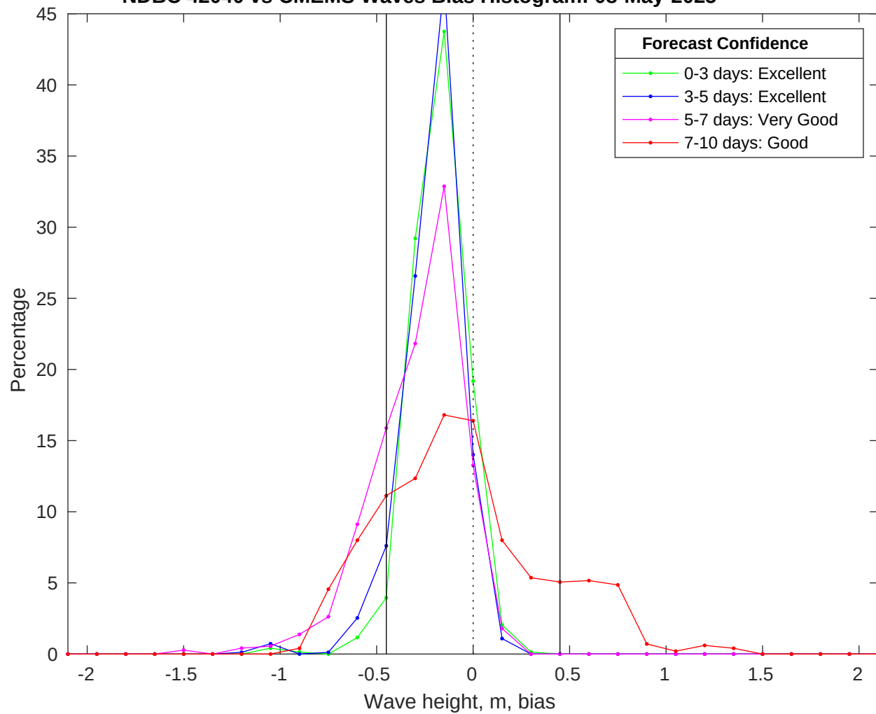
NDBC 42040 vs CMEMS Waves Bias Histogram: 08-May-2025
