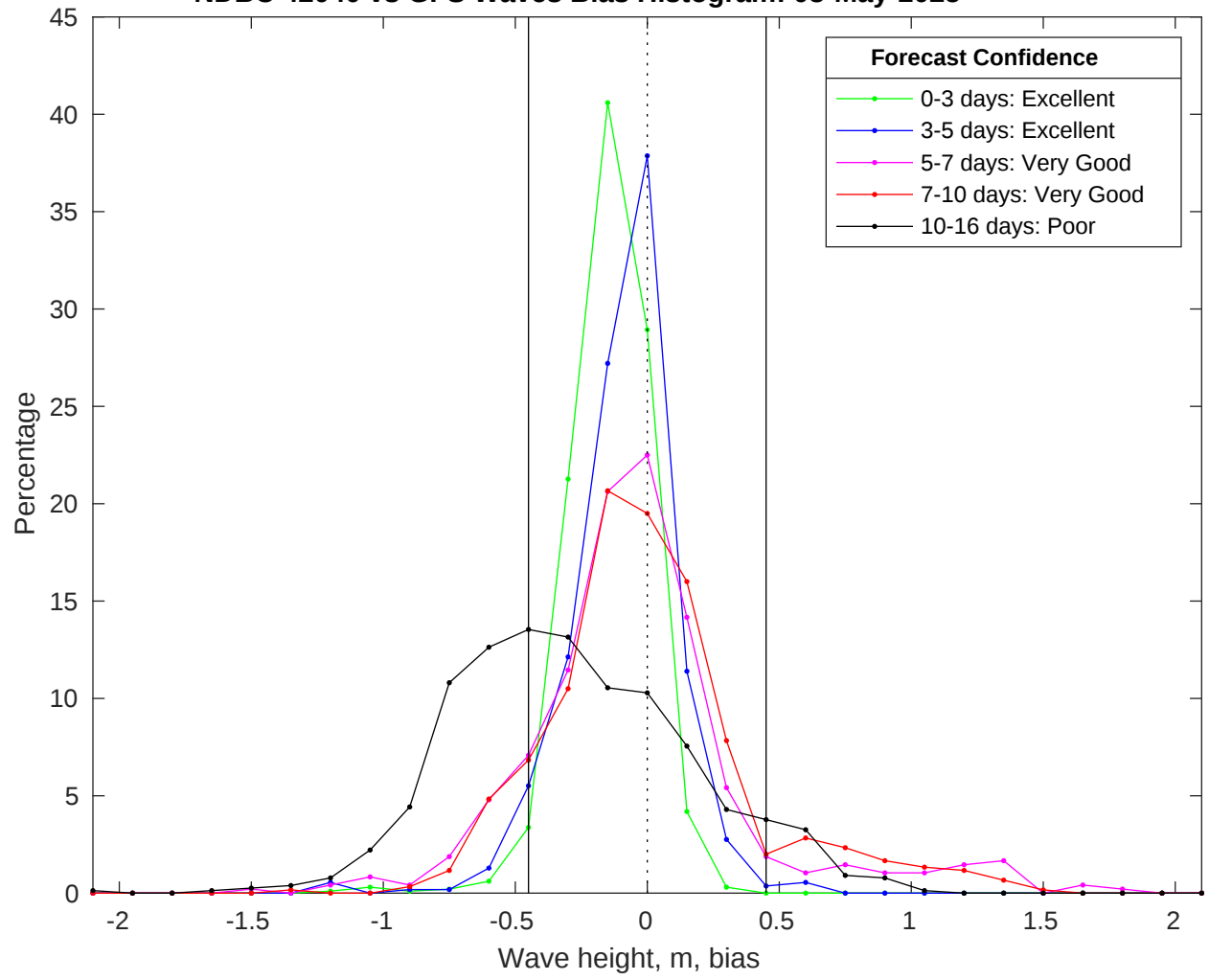
NDBC 42040 vs GFS Waves Bias Histogram: 08-May-2025
