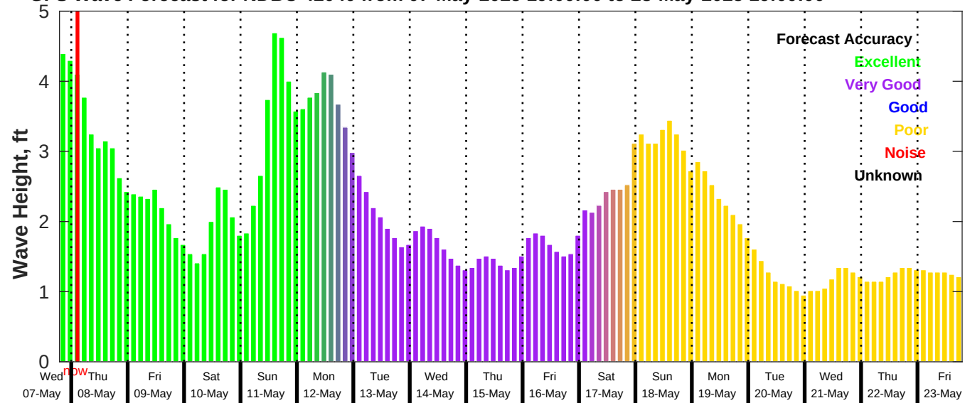
GFS Wave Forecast for NDBC 42040 from 07-May-2025 19:00:00 to 23-May-2025 19:00:00
