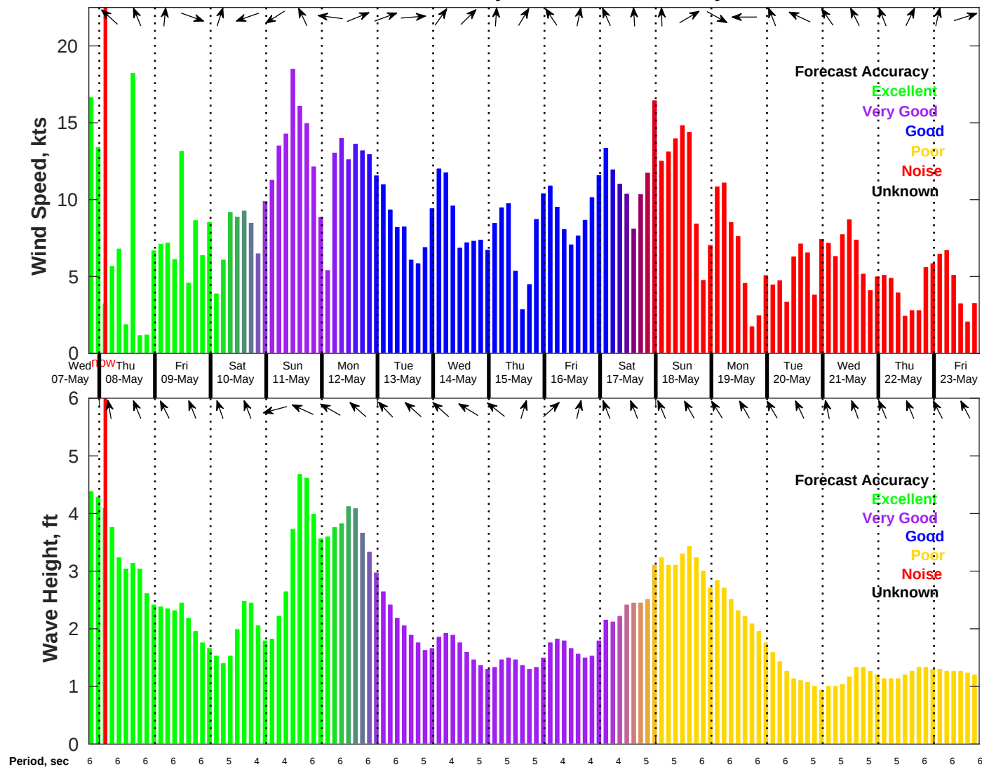
Wind & Wave Forecast for NDBC 42040 from 07-May-2025 19:00:00 to 23-May-2025 19:00:00
