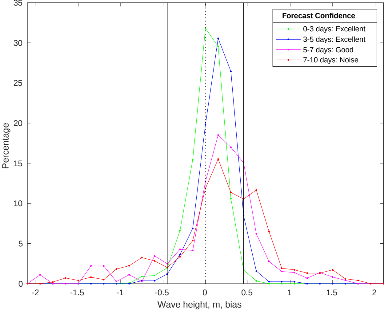
NDBC 46011 vs CMEMS Waves Bias Histogram: 08-May-2025
