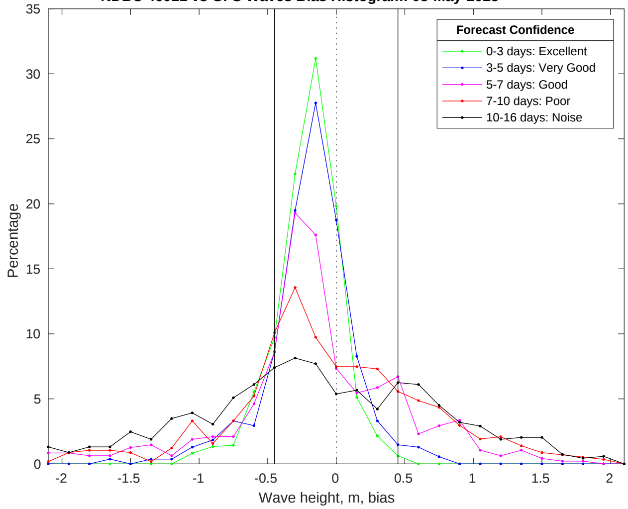
NDBC 46011 vs GFS Waves Bias Histogram: 08-May-2025
