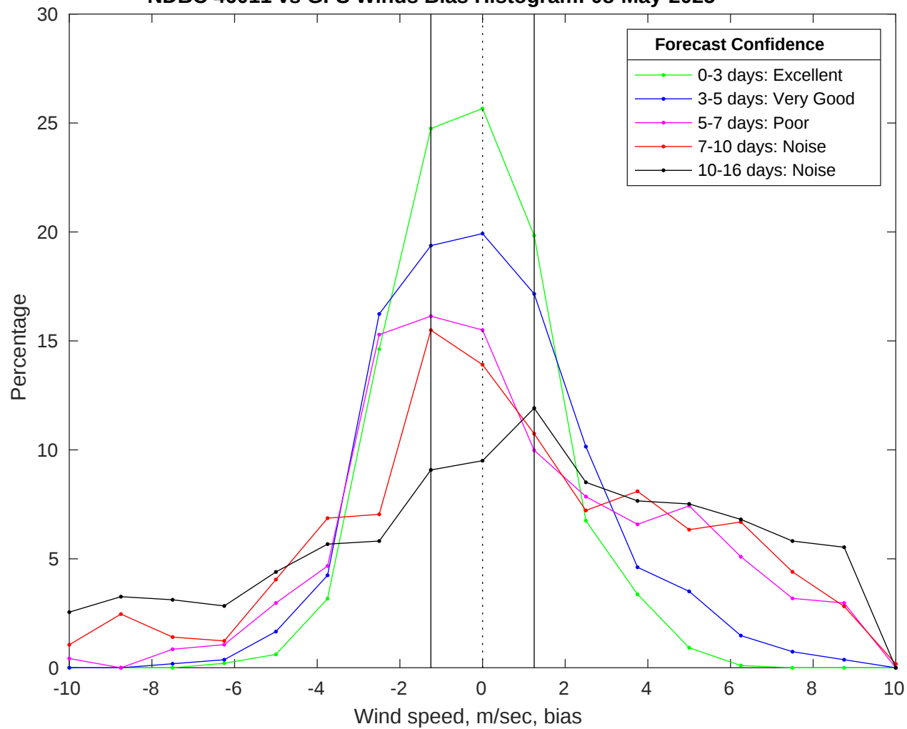
NDBC 46011 vs GFS Winds Bias Histogram: 08-May-2025
