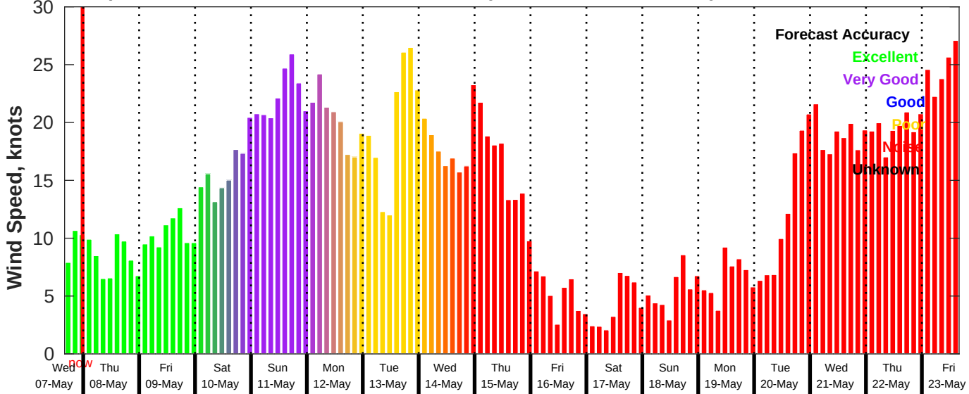
GFS Wind Speed Forecast for NDBC 46011 from 07-May-2025 16:00:00 to 23-May-2025 16:00:00
