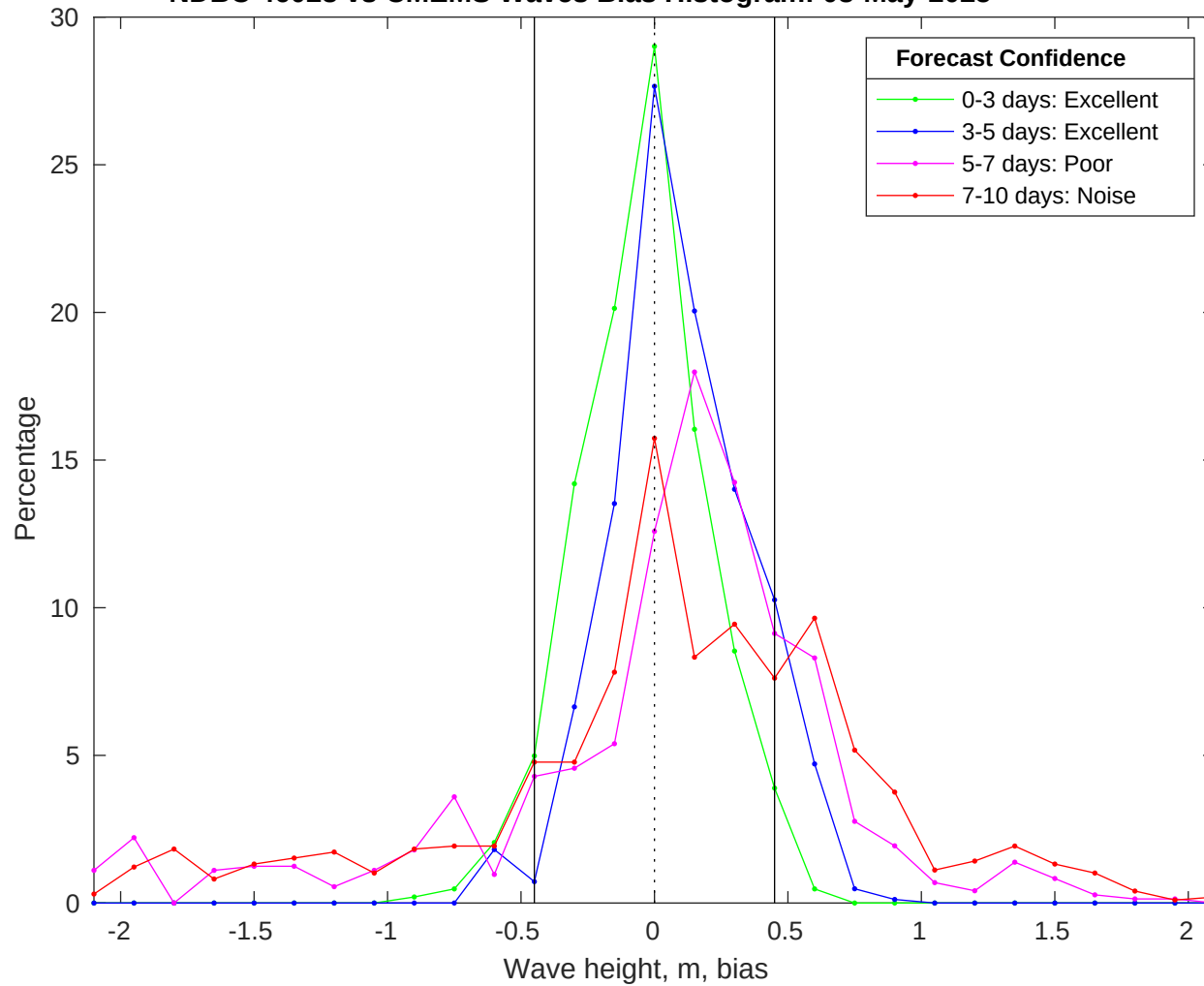
NDBC 46028 vs CMEMS Waves Bias Histogram: 08-May-2025
