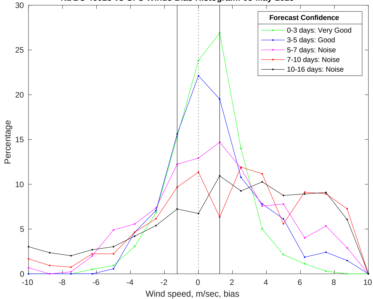
NDBC 46028 vs GFS Winds Bias Histogram: 08-May-2025
