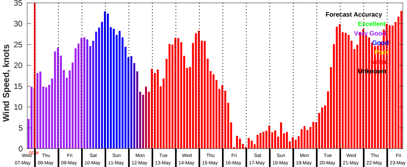
GFS Wind Speed Forecast for NDBC 46028 from 07-May-2025 16:00:00 to 23-May-2025 16:00:00
