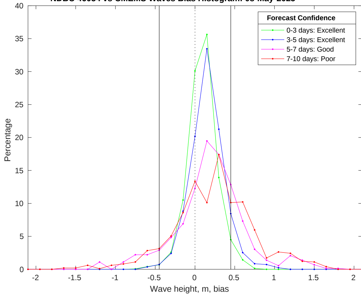
NDBC 46054 vs CMEMS Waves Bias Histogram: 08-May-2025
