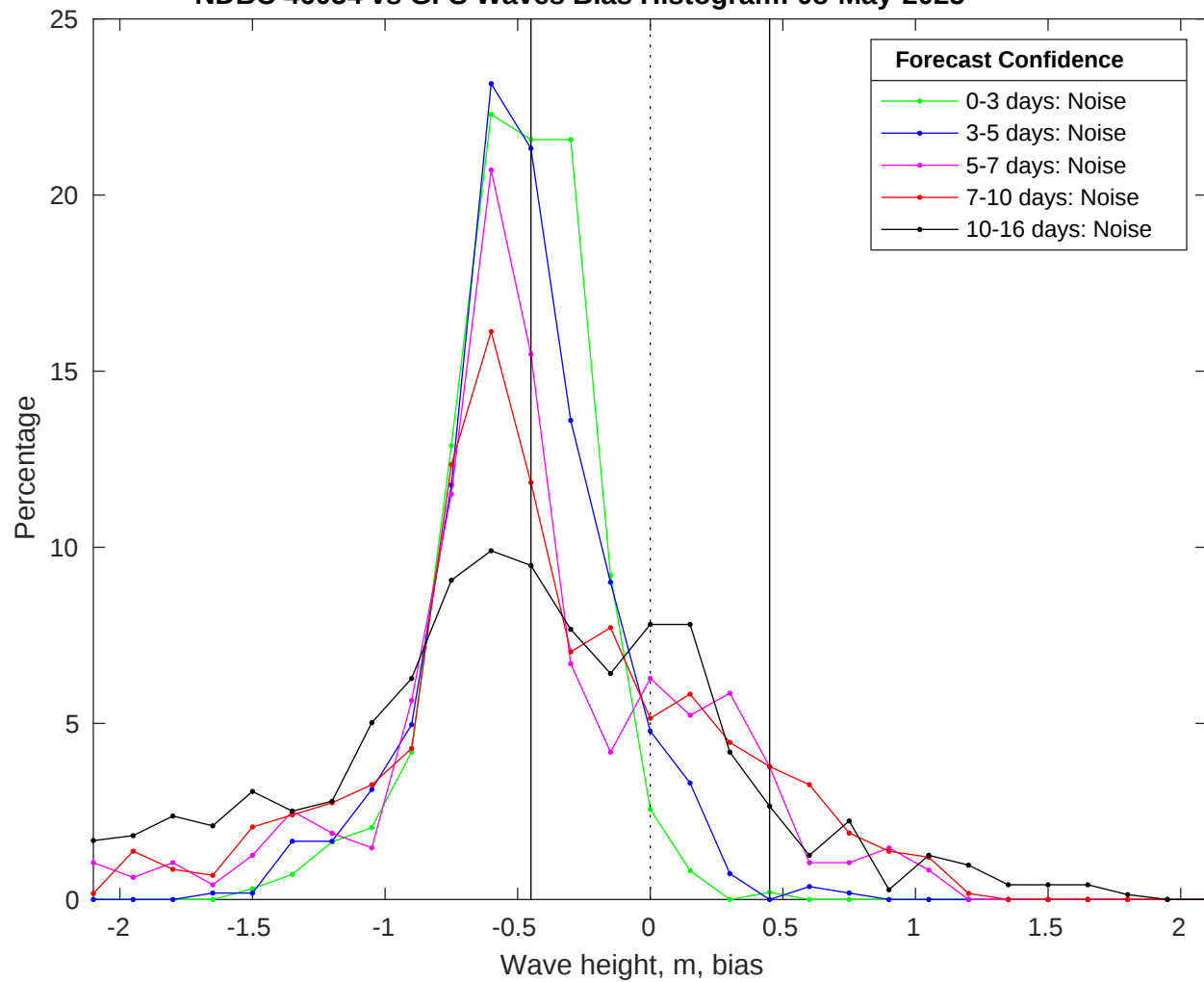
NDBC 46054 vs GFS Waves Bias Histogram: 08-May-2025
