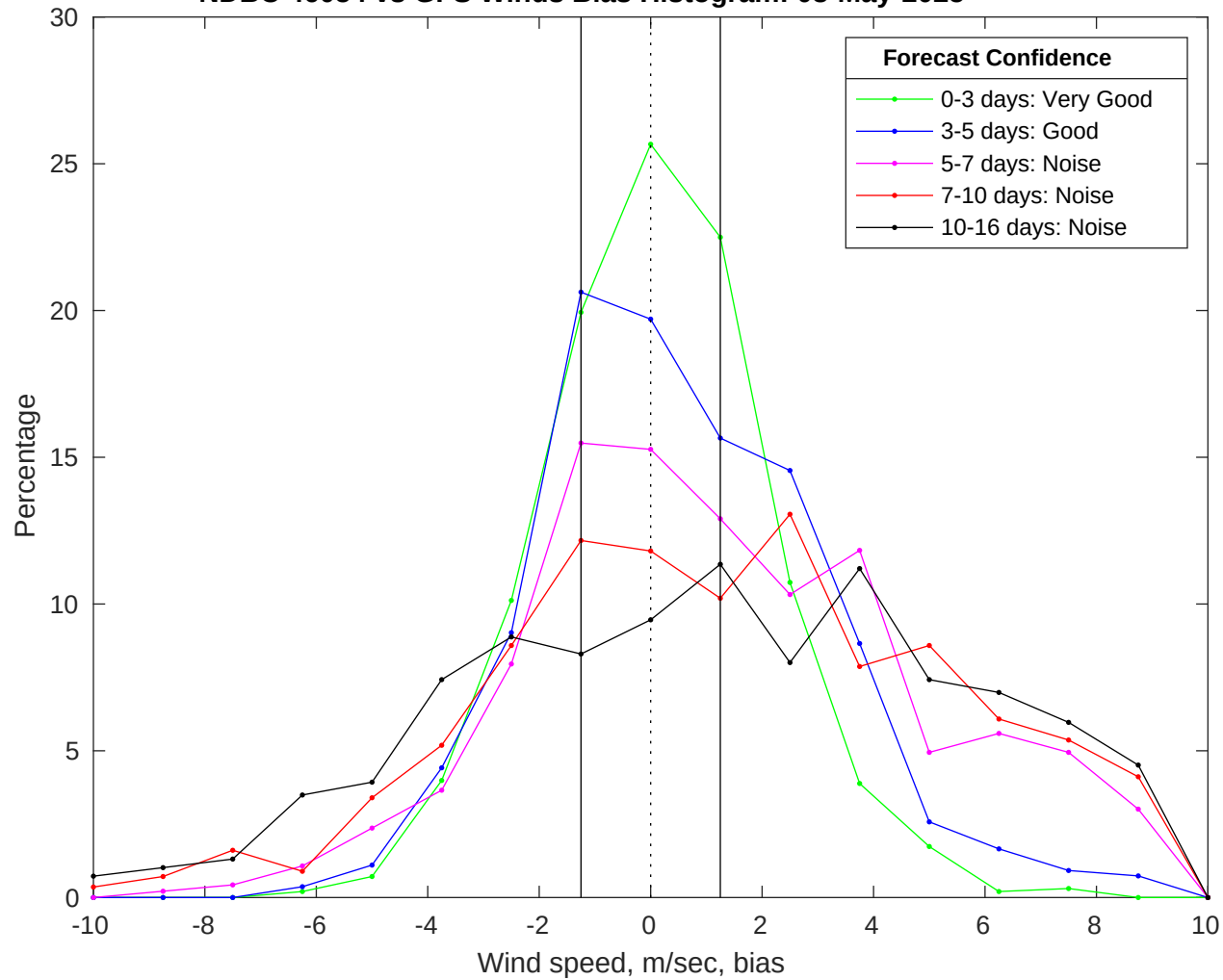
NDBC 46054 vs GFS Winds Bias Histogram: 08-May-2025
