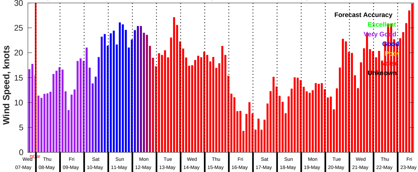
GFS Wind Speed Forecast for NDBC 46054 from 07-May-2025 16:00:00 to 23-May-2025 16:00:00
