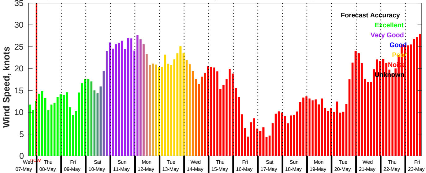
GFS Wind Speed Forecast for NDBC 46069 from 07-May-2025 16:00:00 to 23-May-2025 16:00:00
