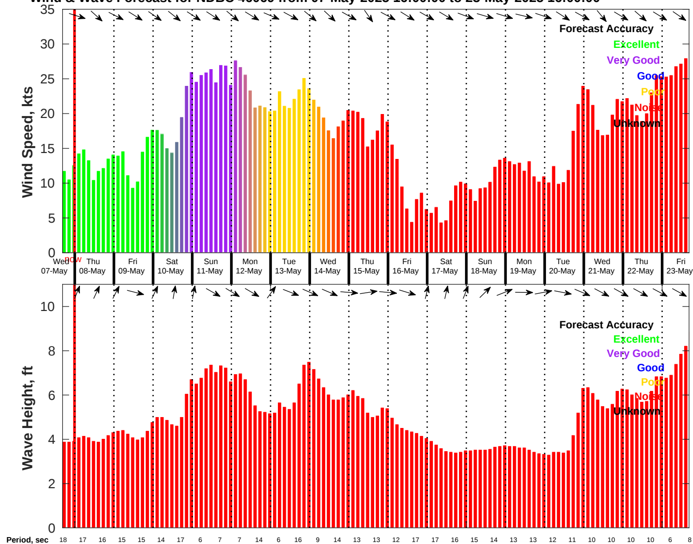
Wind & Wave Forecast for NDBC 46069 from 07-May-2025 16:00:00 to 23-May-2025 16:00:00
