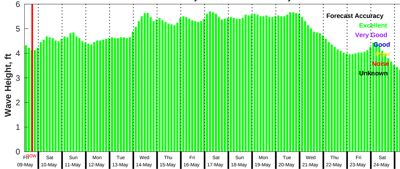
GFS Wave Forecast for NDBC 52211 from 08-May-2025 10:00:00 to 24-May-2025 10:00:00
