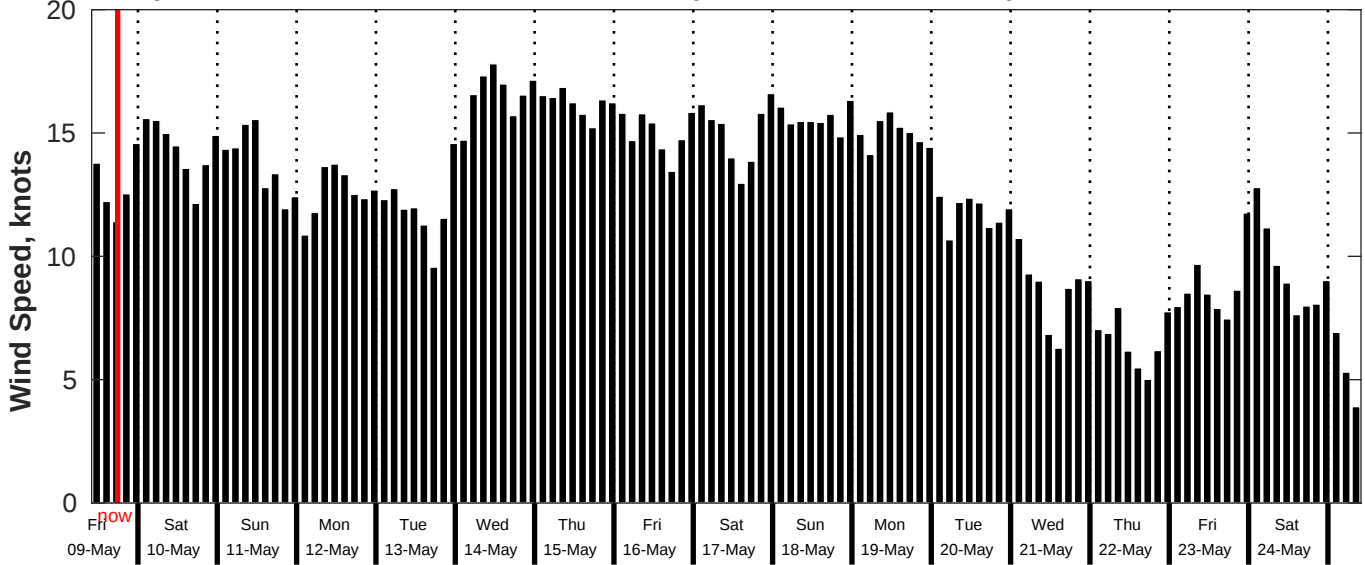
GFS Wind Speed Forecast for NDBC 52211 from 08-May-2025 10:00:00 to 24-May-2025 10:00:00
