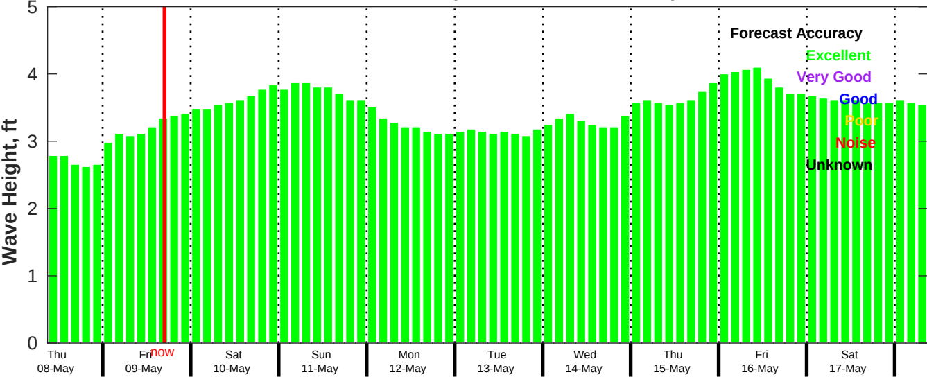
CMEMS Wave Forecast for NDBC 52212 from 07-May-2025 09:00:00 to 17-May-2025 09:00:00
