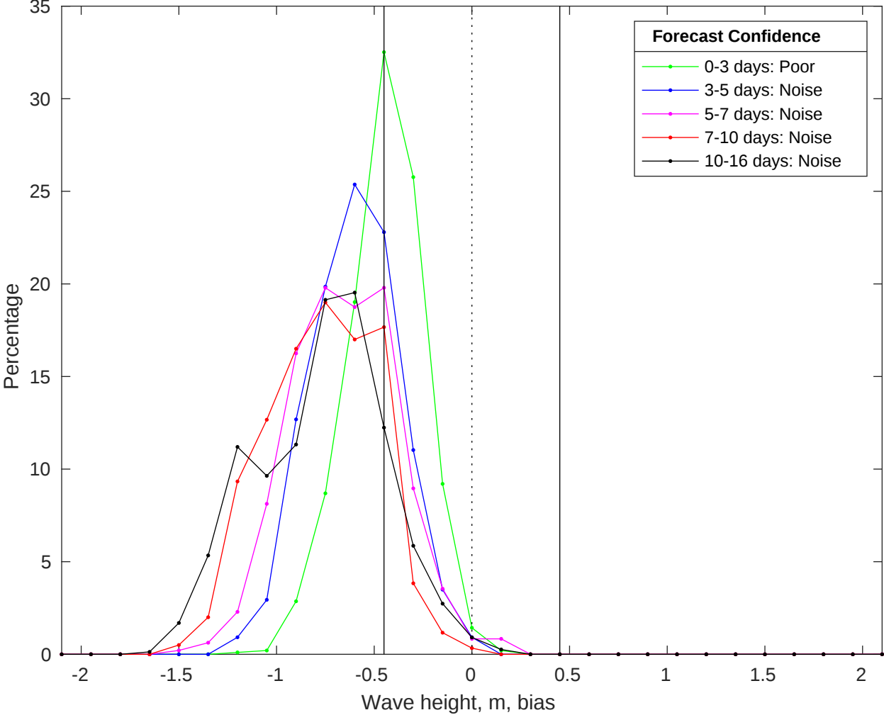
NDBC 52213 vs GFS Waves Bias Histogram: 08-May-2025
