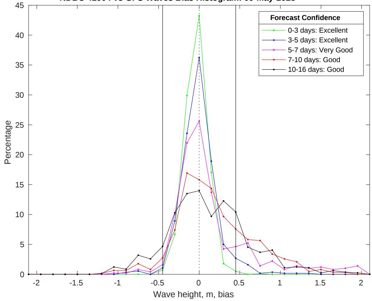
NDBC 41004 vs GFS Waves Bias Histogram: 09-May-2025
