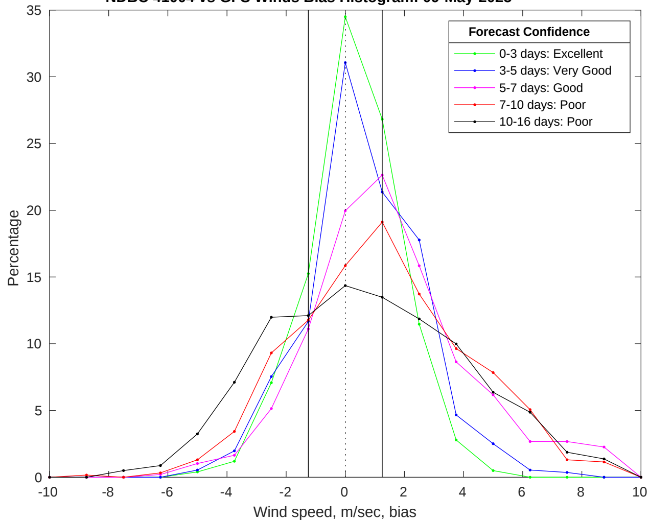
NDBC 41004 vs GFS Winds Bias Histogram: 09-May-2025
